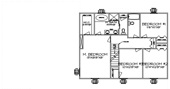
SECOND FLOOR PLAN SCALE: 1/4"=1'-0"
