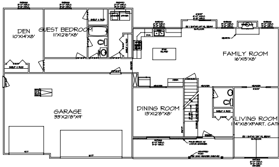
FIRST FLOOR PLAN SCALE: 1/4"=1'-0"
